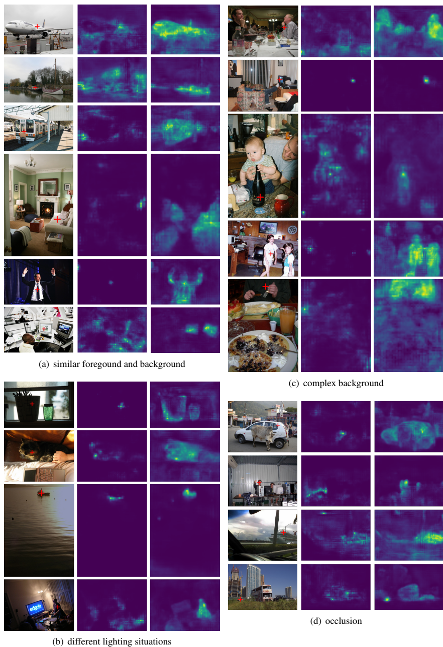
Figure 2: Visualization of LGSA using challenging images. The first column is origin images, the second column is Non-local’s results and the last column is ours. The query point is marked as a red ‘+’ and the corresponding weights are sampled from the affinity matrix and shown as a heatmap.
