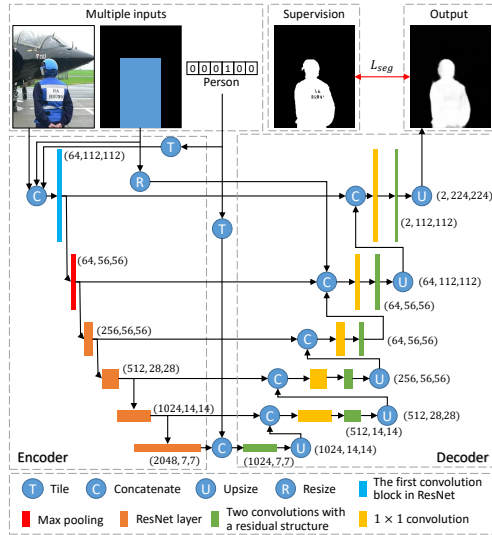
Figure 1: The detailed structure of CFS network.
